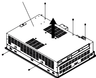
PS-A unit's Rear Cover
