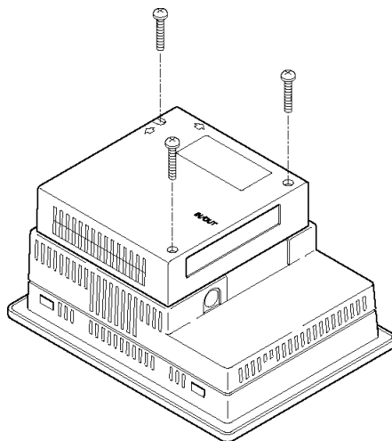
GLC-100 Unit
